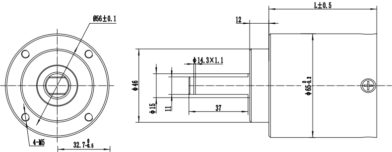
外型图/ Mechanical Dimension
